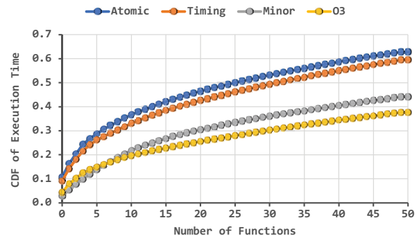
Fig. 15: Top 50 hottest functions in gem5 when simulating a PARSEC workload with different CPU types.
