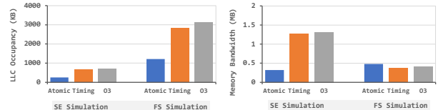
Fig. 9: LLC occupancy and memory bandwidth utilization of gem5 running with different configurations and operating modes on Intel_Xeon.
